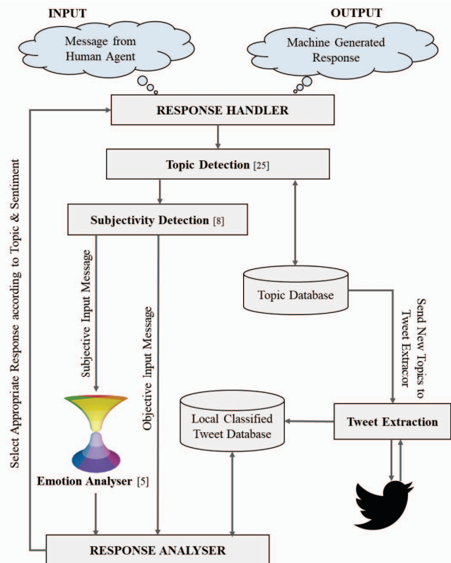
Fig. 2. Proposed Framework
