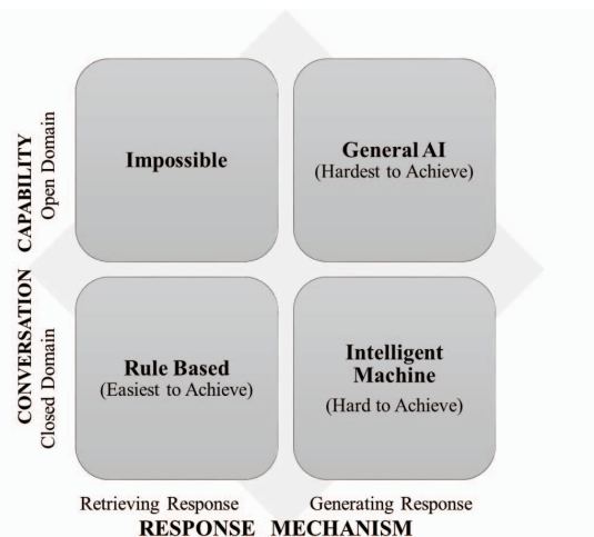
Fig. 1. Categories of dialog system research
