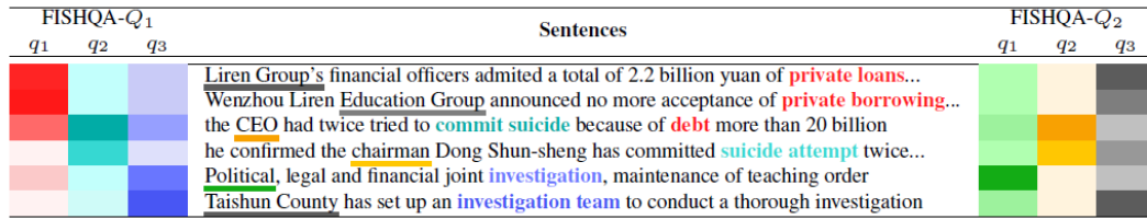
Fig. 10. FISHQA: hierarchical attention model, different colors relating to different financial concepts, grey - company, light brown - executives, red - financing, blue - litigation, teal - personnel. [75].
